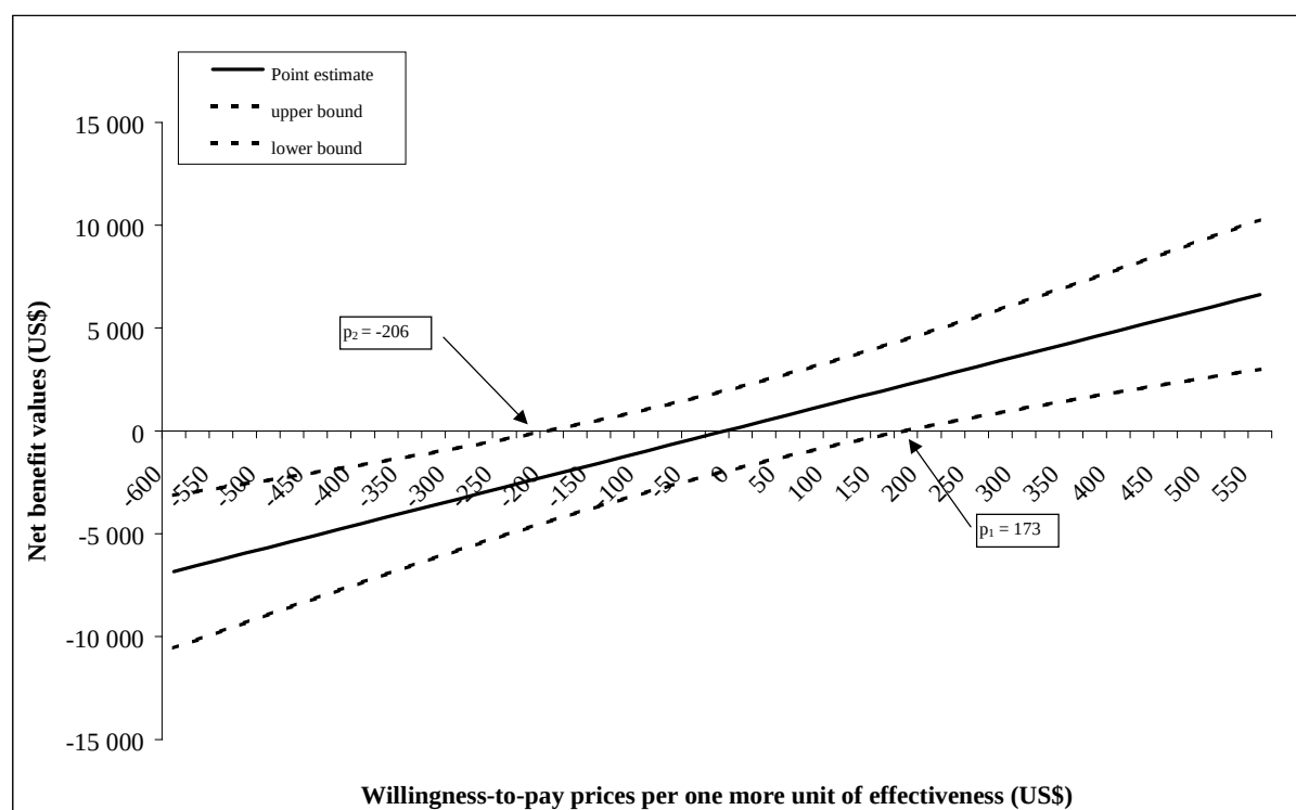
Figure 2. Confidence intervals for the net benefit for different willingness to pay prices.
