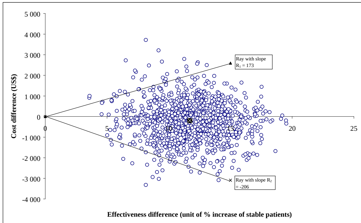
Figur 1. ICER bootstrap replicates and 95% Fieller confidence limits for the ICER.
